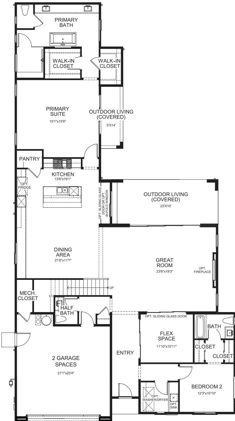
FIRST FLOOR
