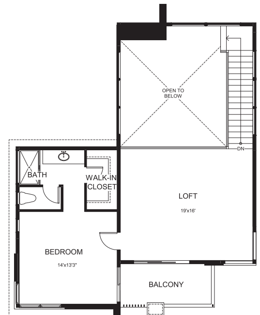
SECOND FLOOR PRIVATE GUEST SUITE
